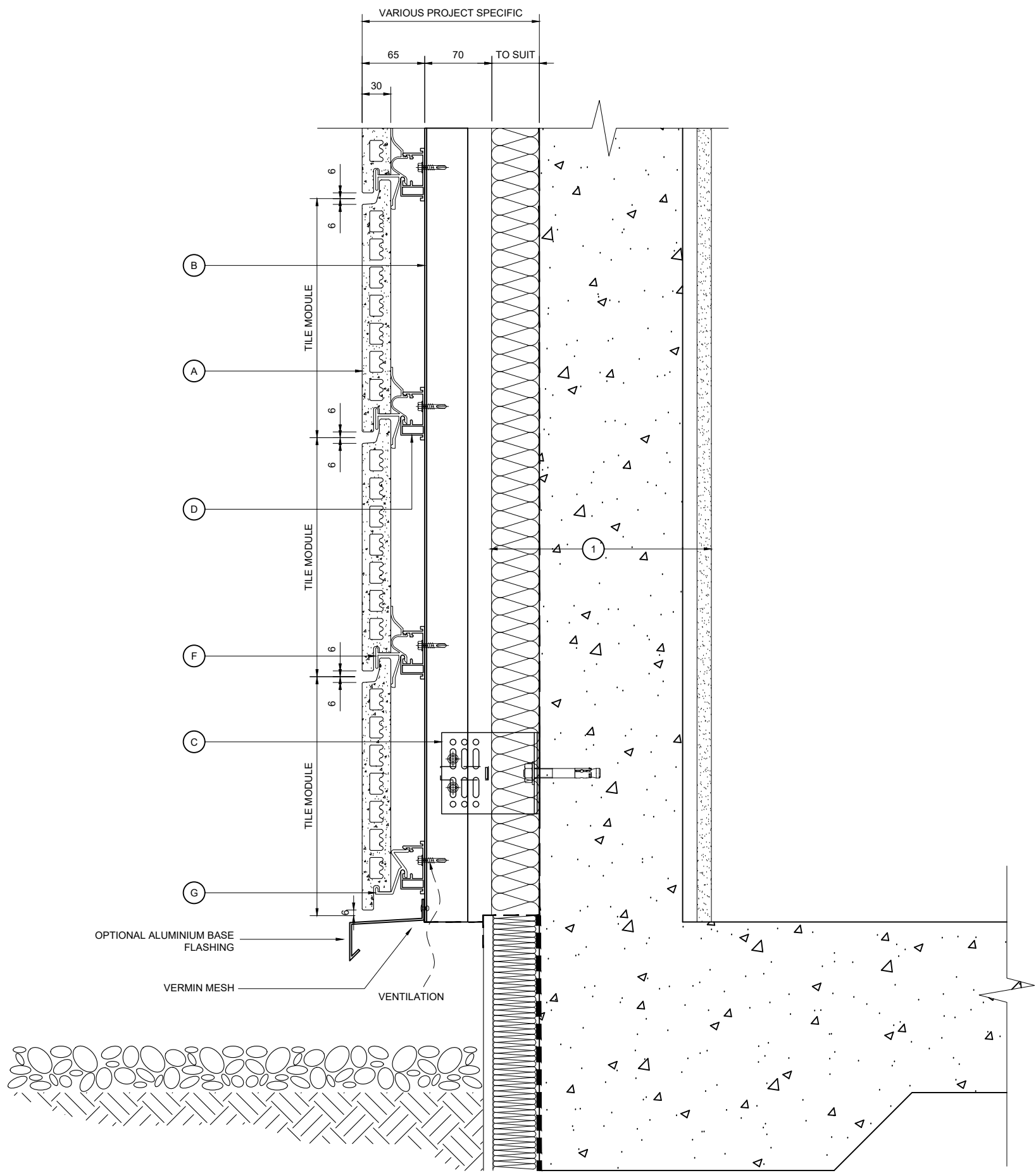
BASE DETAIL
