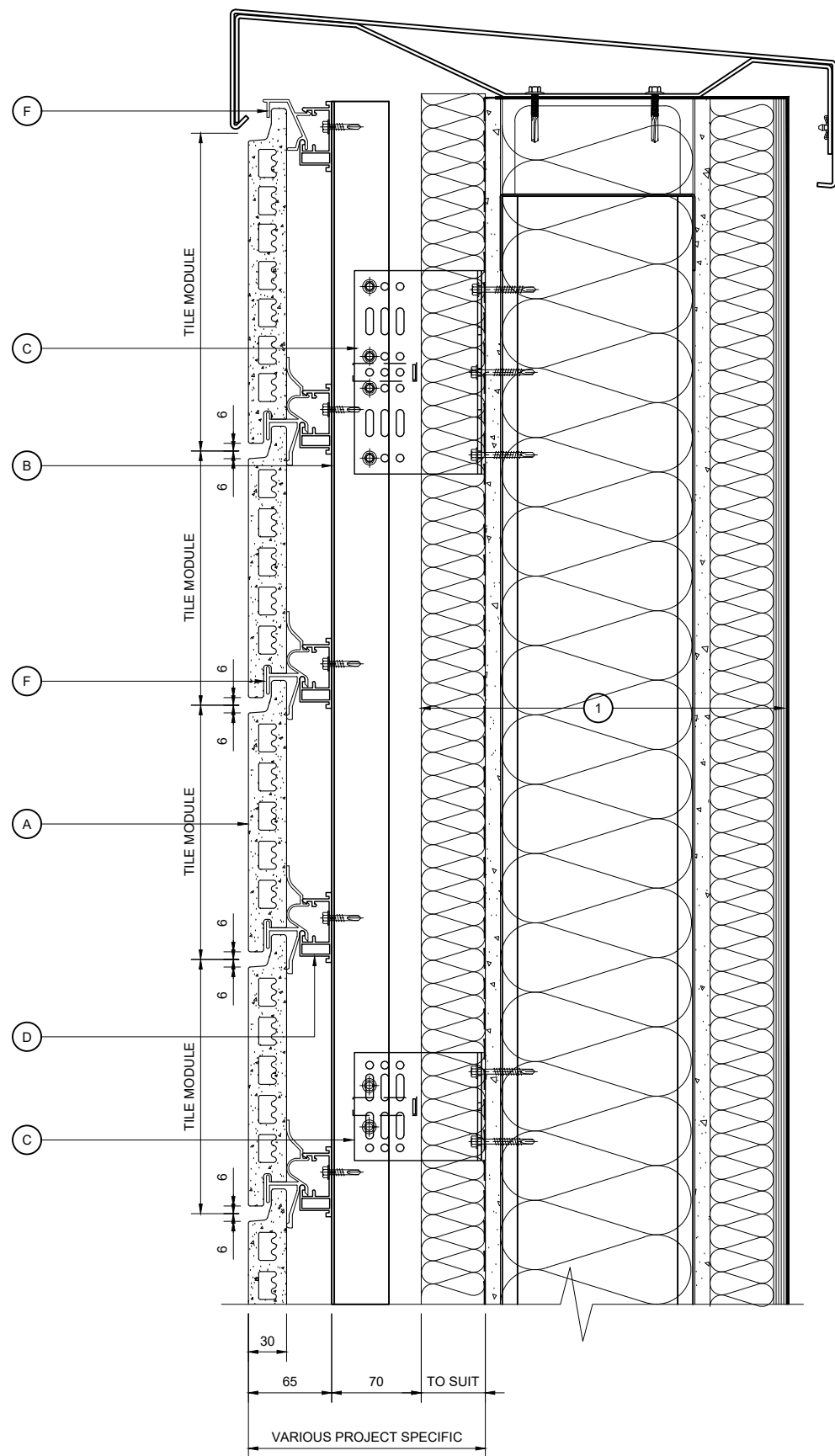
PARAPET DETAIL
