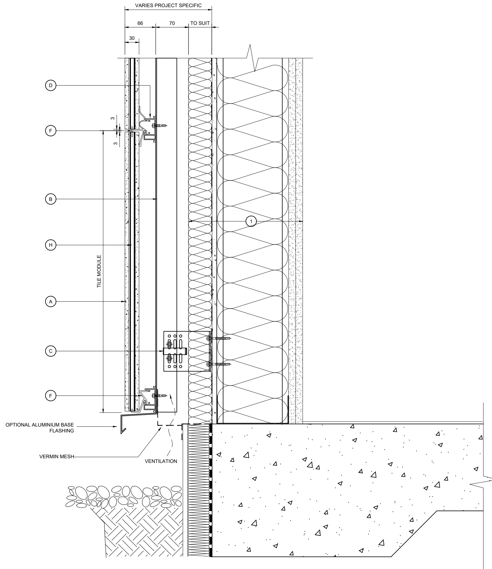
BASE DETAIL
